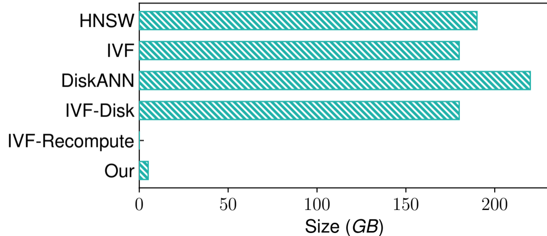
Storage Usage
