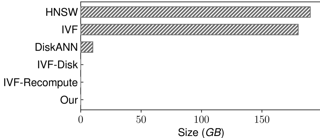
RAM Usage
